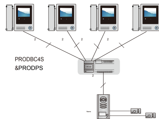
Star topology:
