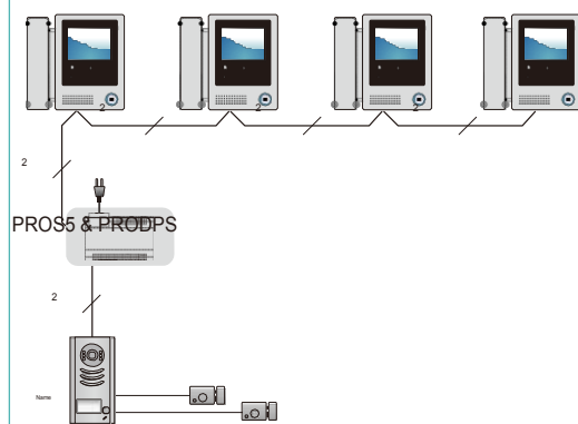
In-Out topology:
